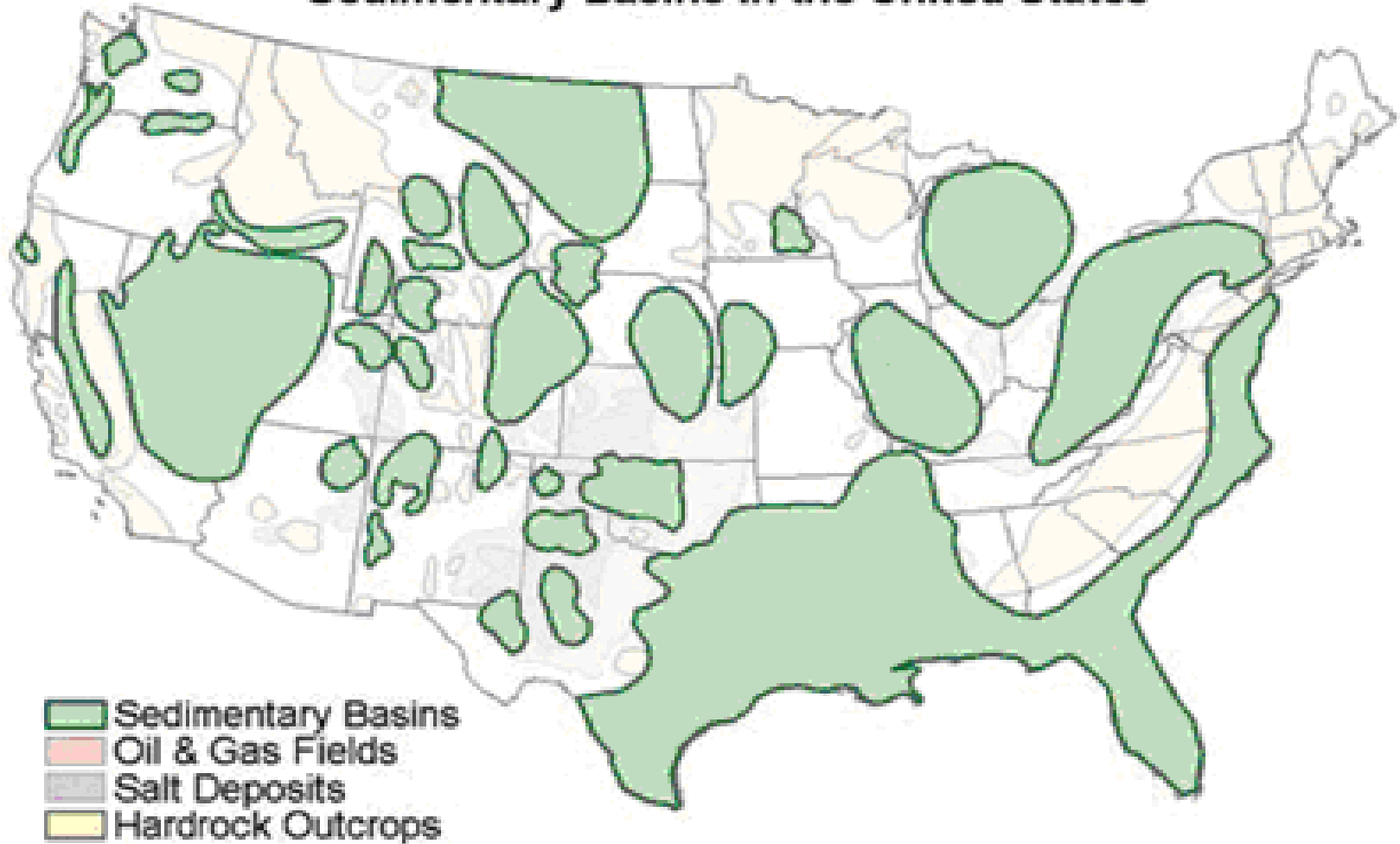
Sedimentary Basins in the United States
